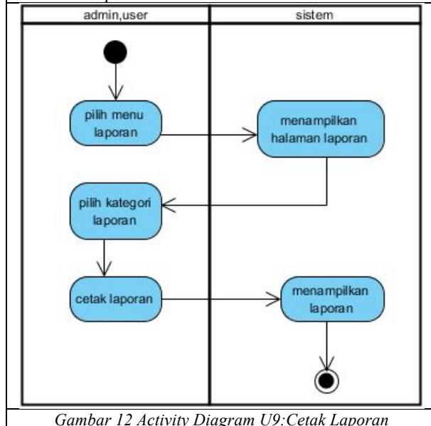
Gambar 12 Activity Diagram U9:Cetak Laporan
