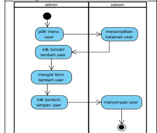
Gambar 13 Activity Diagram U10:Mengelola User
