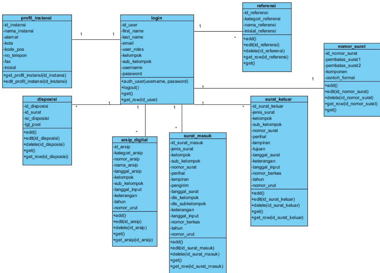
Gambar Diagram Class Digital Archiving
