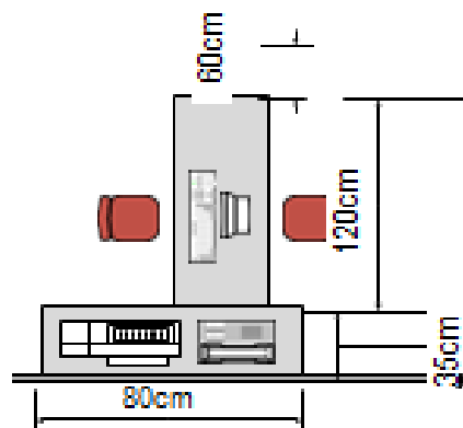
Gambar 17. Layout Raw Material (ruangan lama)
